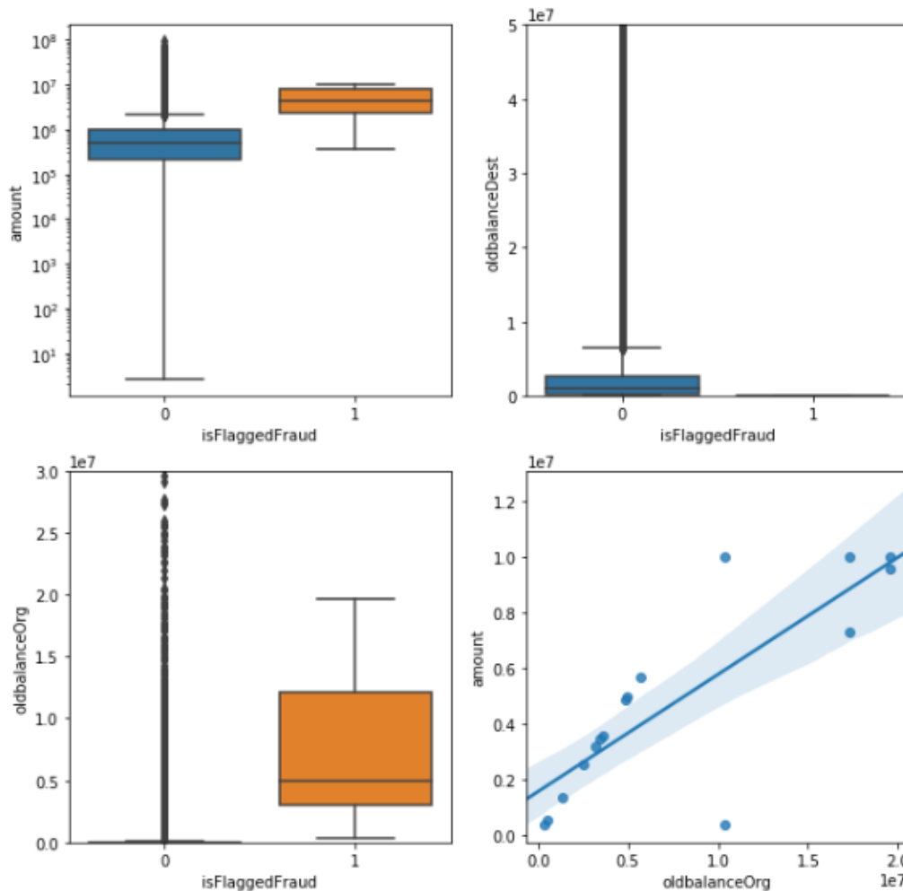
Figure 26: scikit-learn
