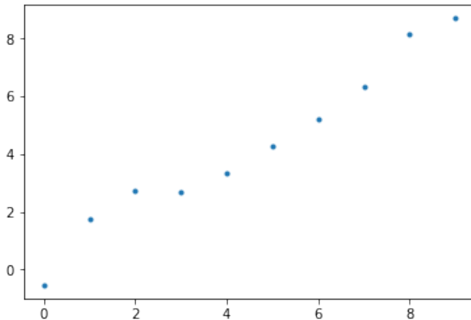
Figure 21: Result 1
