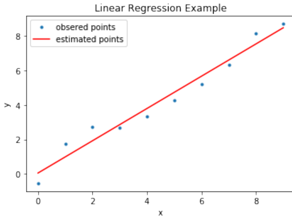
Figure 22: Result 2
