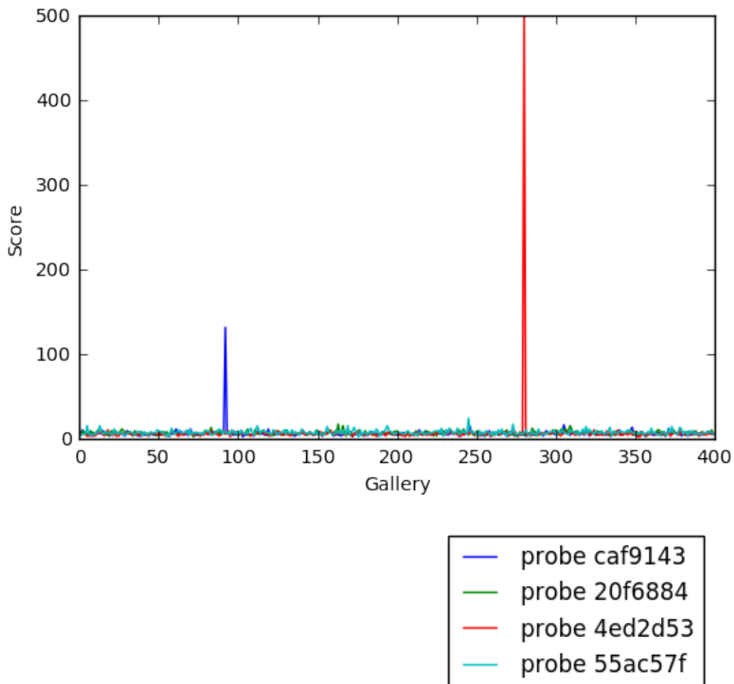
Figure 36: Result
