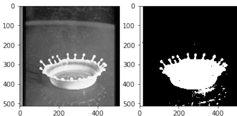
Figure 5: Image Thresholding
