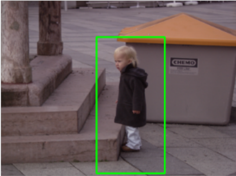
Figure 39: Pedestrian Detected
