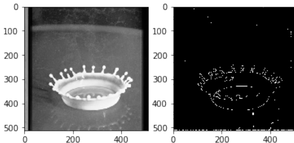
Figure 6: Edge detection
