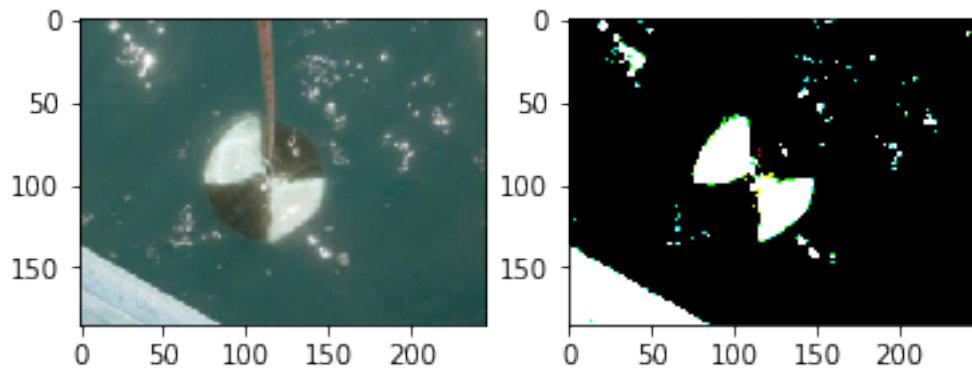
Figure 9: Threshold 1, threshold(img1)
