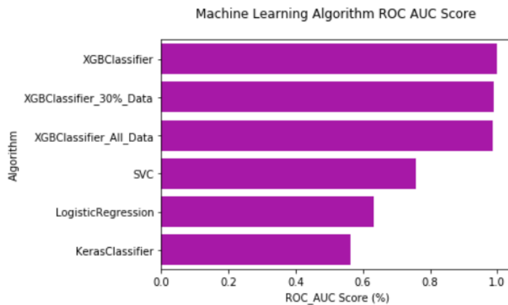
Figure 31: scikit-learn
