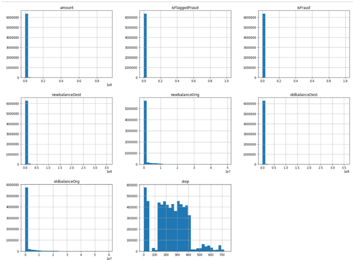
Figure 25: scikit-learn
