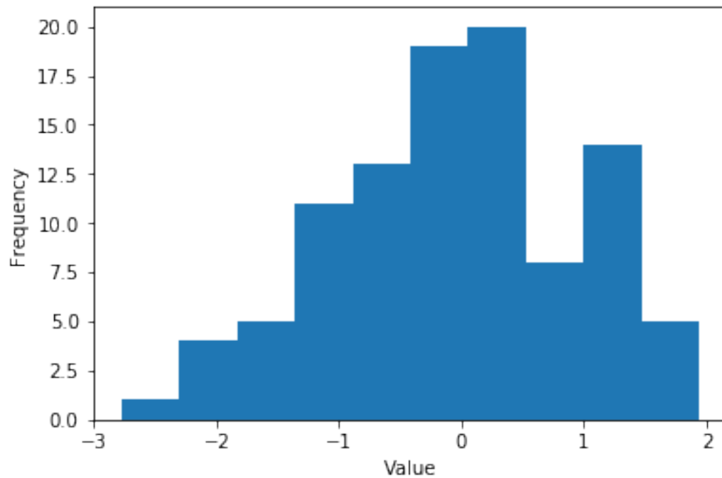
Figure 20: Histogram 3
