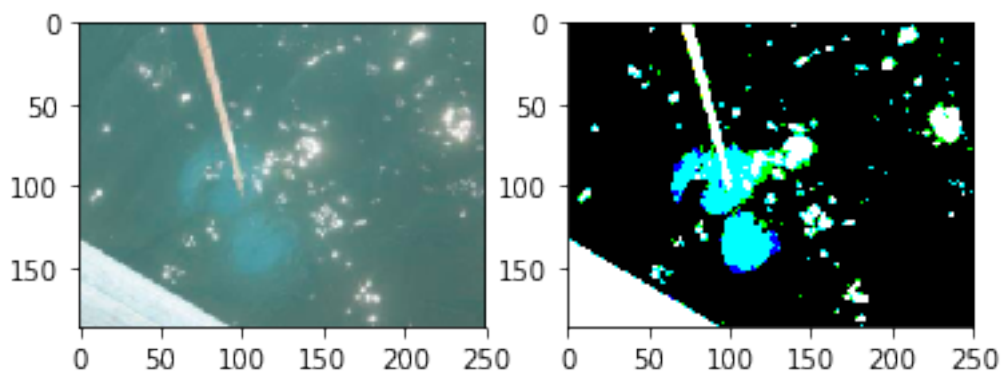
Figure 11: Threshold 3, threshold(img3)
