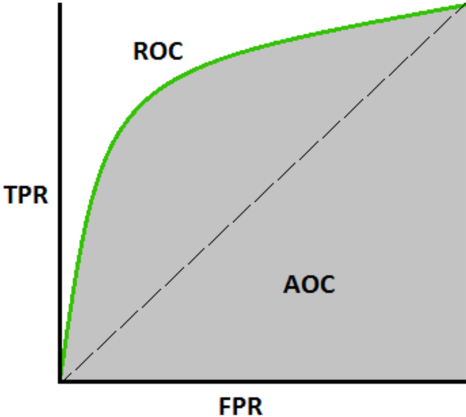
Figure 30: scikit-learn
