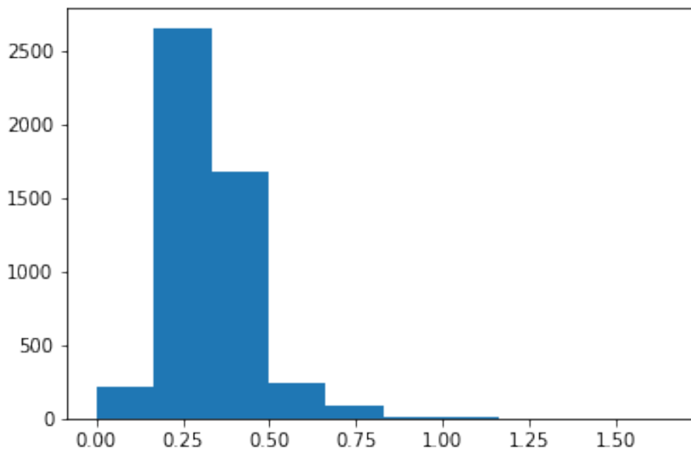
Figure 33: Histogram
