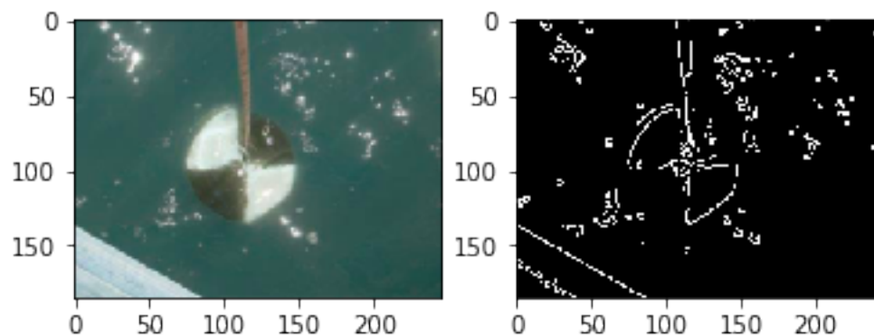
Figure 13: Edge Detection 1, find_edge(img1)
