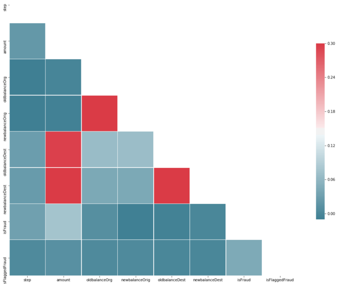
Figure 24: scikit-learn correlation array
