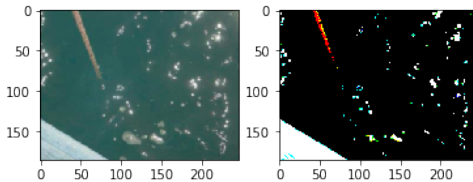
Figure 12: Threshold 4, threshold(img4)
