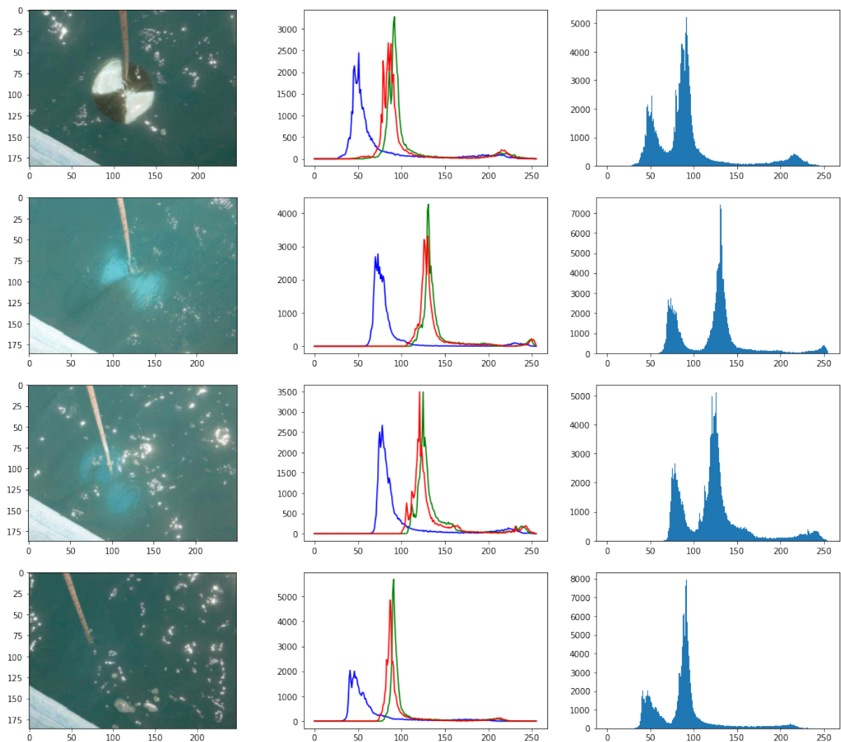
Figure 8: Histogram
