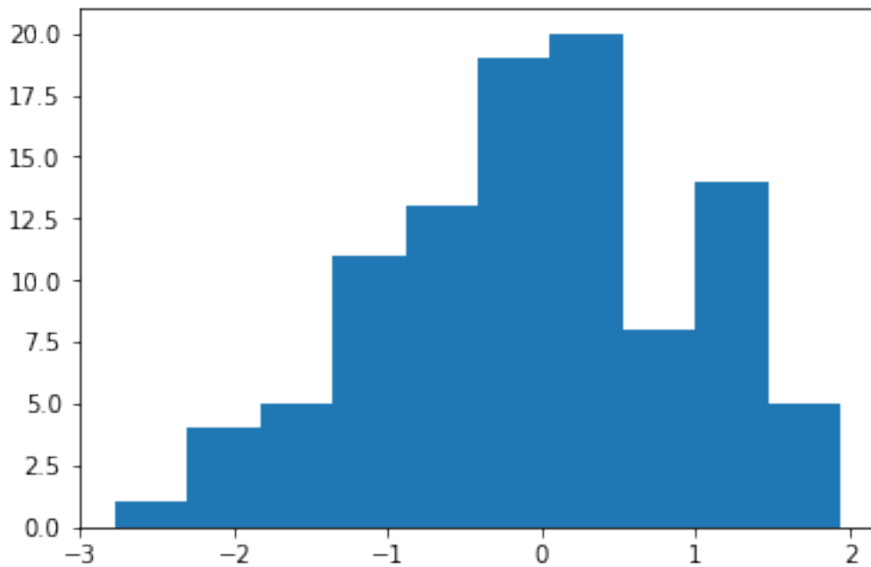
Figure 18: Histogram 1
