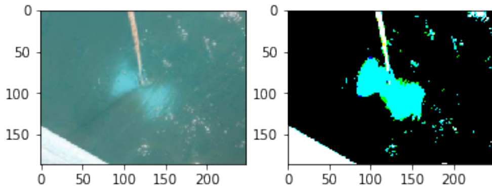
Figure 10: Threshold 2, threshold(img2)
