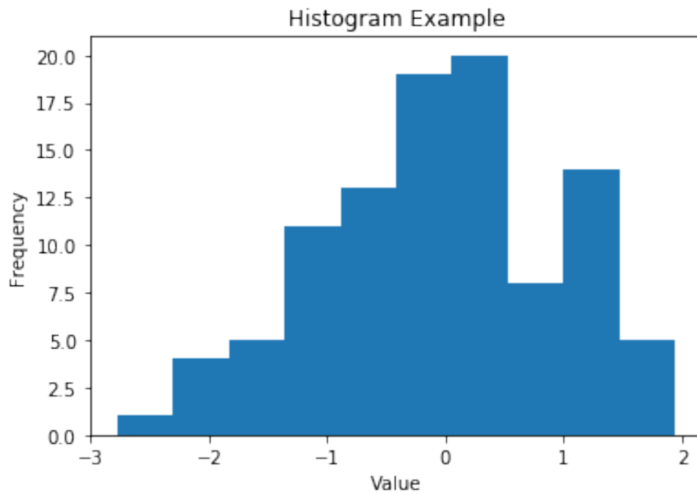
Figure 19: Histogram 2
