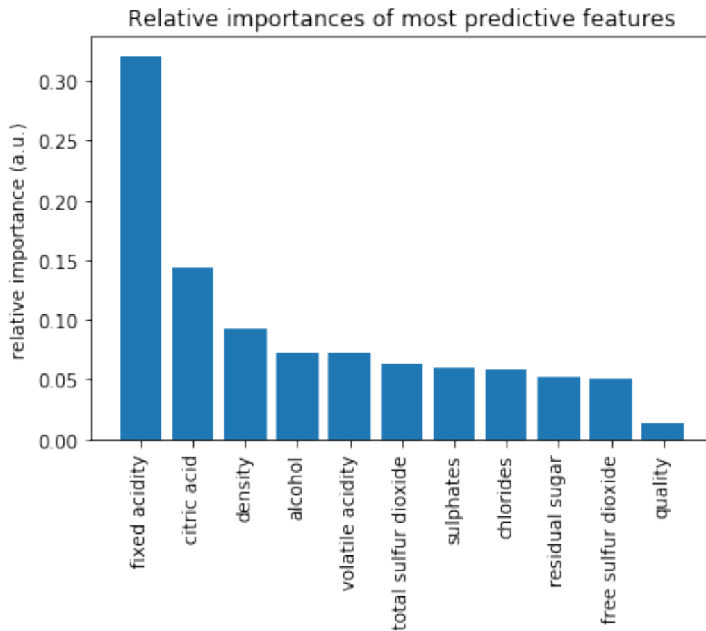
Figure 34: Result
